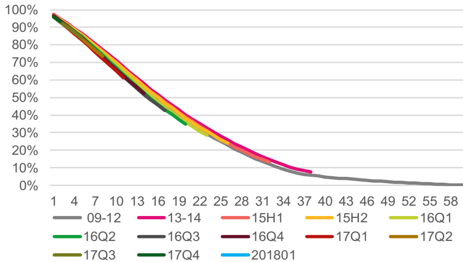
Remaining Balance (%)
